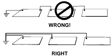
Figure 3. ESD work surfaces should never be grounded in series, i.e. daisy chained.
