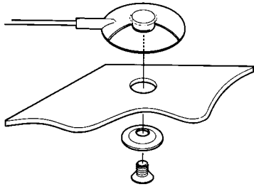
Figure 11. Installing 60474/60488 to mat using supplied hardware.
