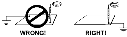
Figure 5. Proper grounding of wrist straps.
