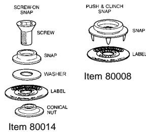
Figure 7. Two kinds of snaps.
