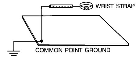
Figure 4. Common point ground for each workstation.
