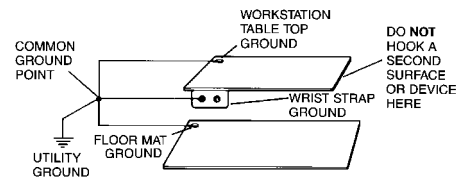
Figure 10. 60354 dual bench mount.
