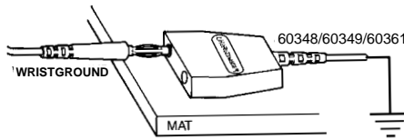
Figure 12. Adding the wriststrap.
